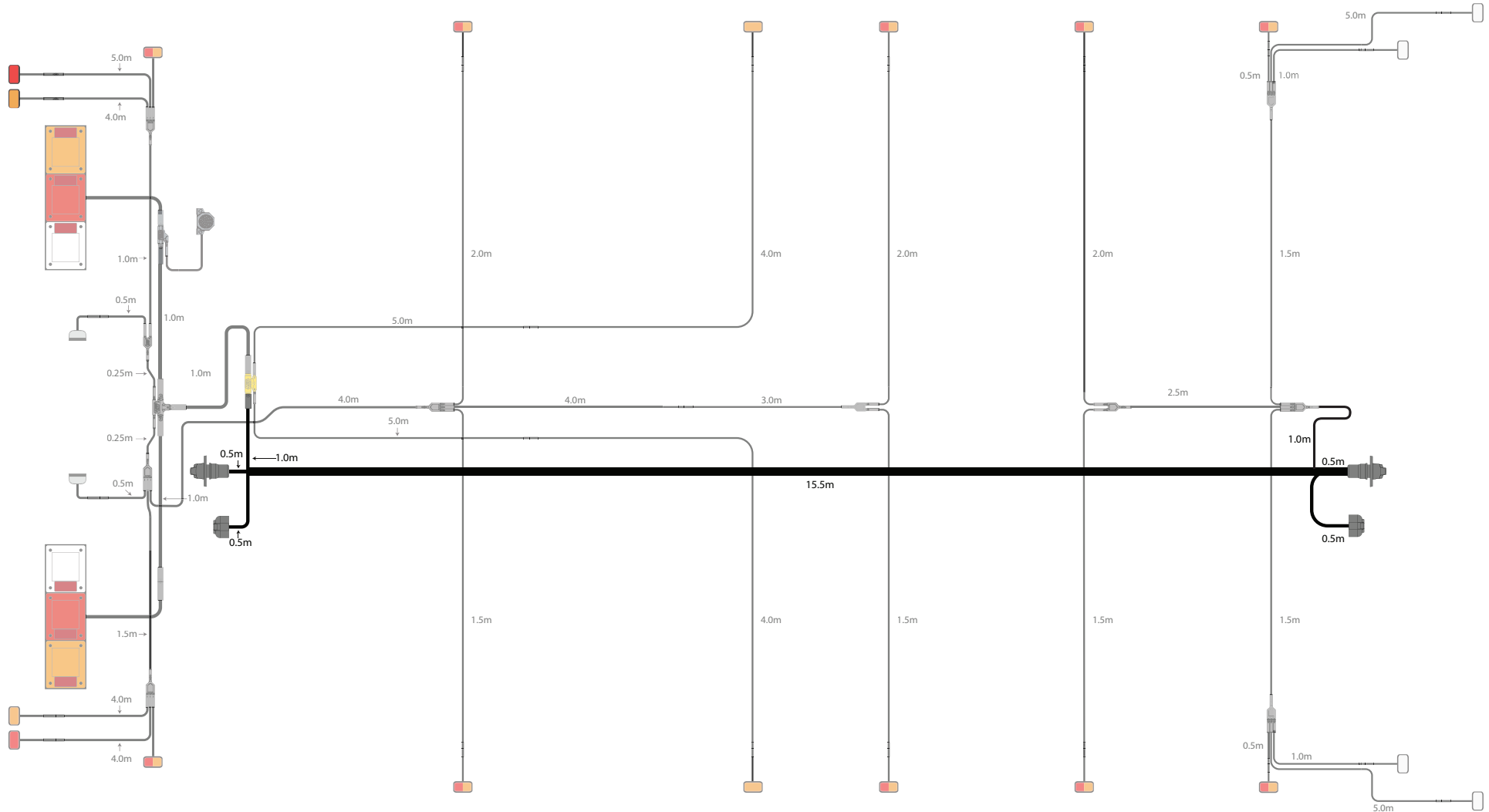
DROPDECK SCHEMATIC EXAMPLE ROAD TRAIN CABLE
