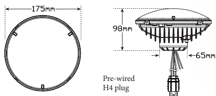
Road Legal Low Beam HL175
